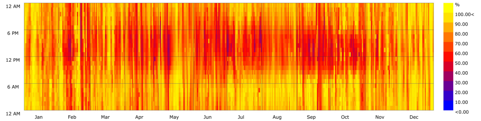
Relative Humidity (%) - Hourly ISTANBUL_TUR 1 JAN 1:00 - 31 DEC 24:00
