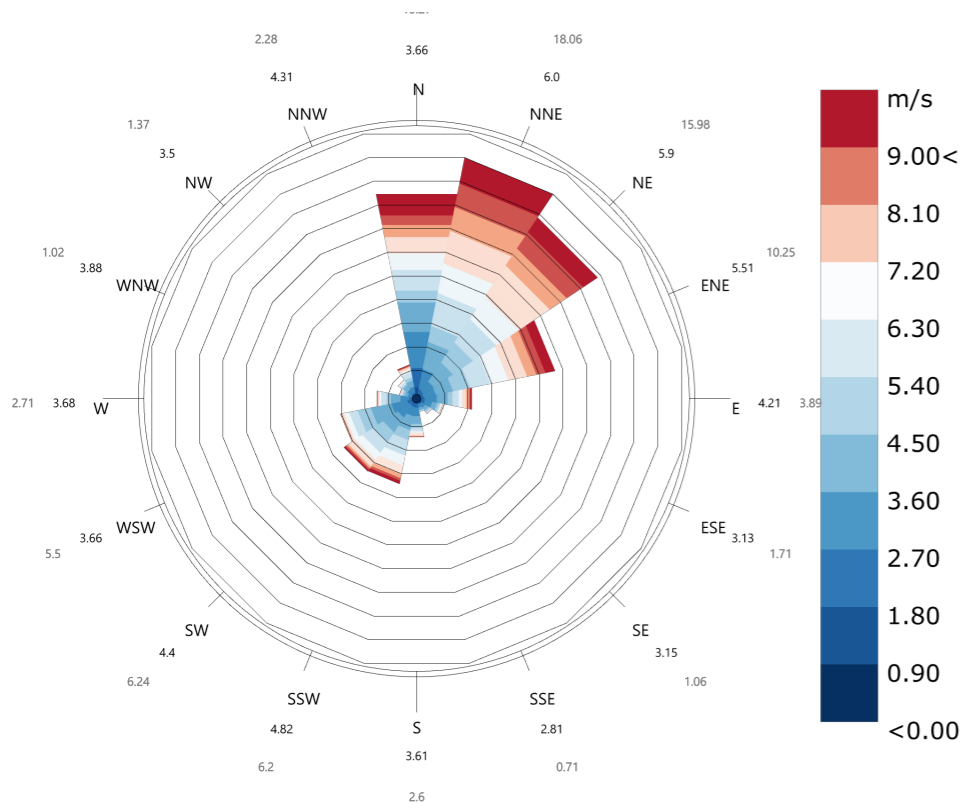
Wind-Rose ISTANBUL_TUR 1 JAN 1:00 - 31 DEC 24:00 Hourly Data: Wind Speed (m/s) Calm for 5.14% of the time = 450 hours. Each closed polyline shows frequency of 1.8%. = 158 hours.
